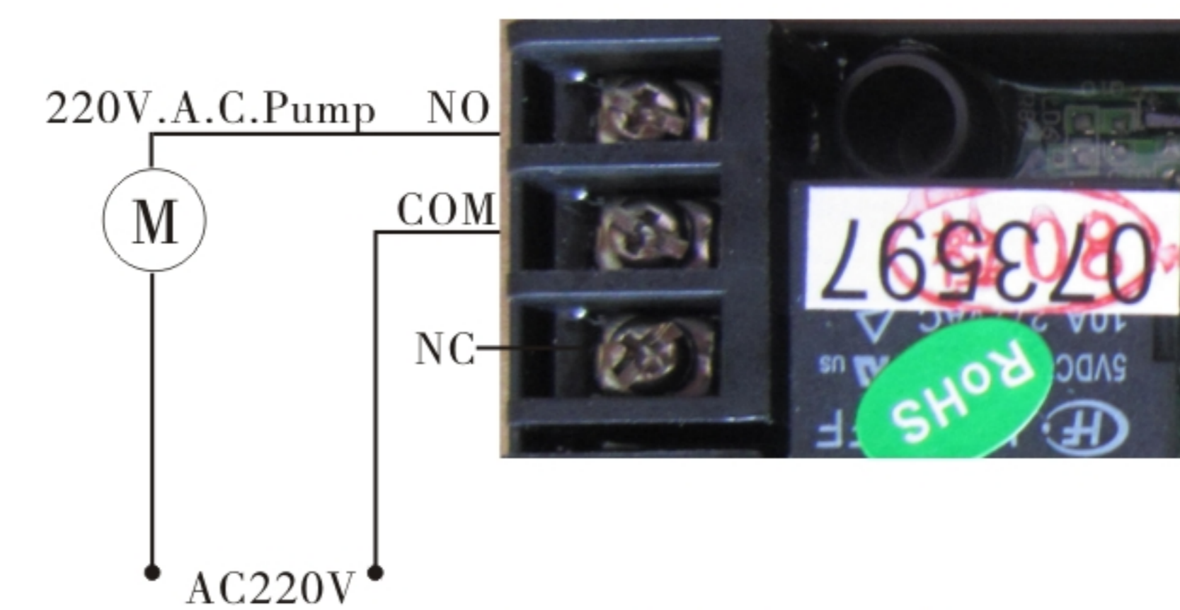
Figure 3-6Wiring of Booster pump on Inlet
