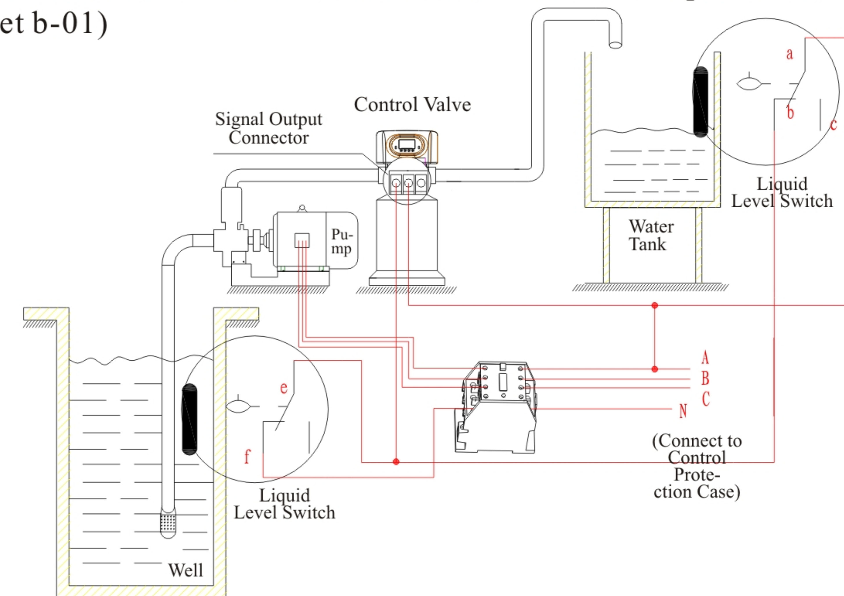
Figure3-5Wiring of Liquid Level controller controlling Inlet Pump
