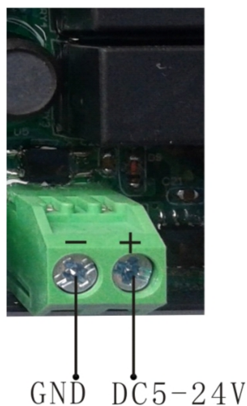
Figure 3-9 Wiring of Remote Input
