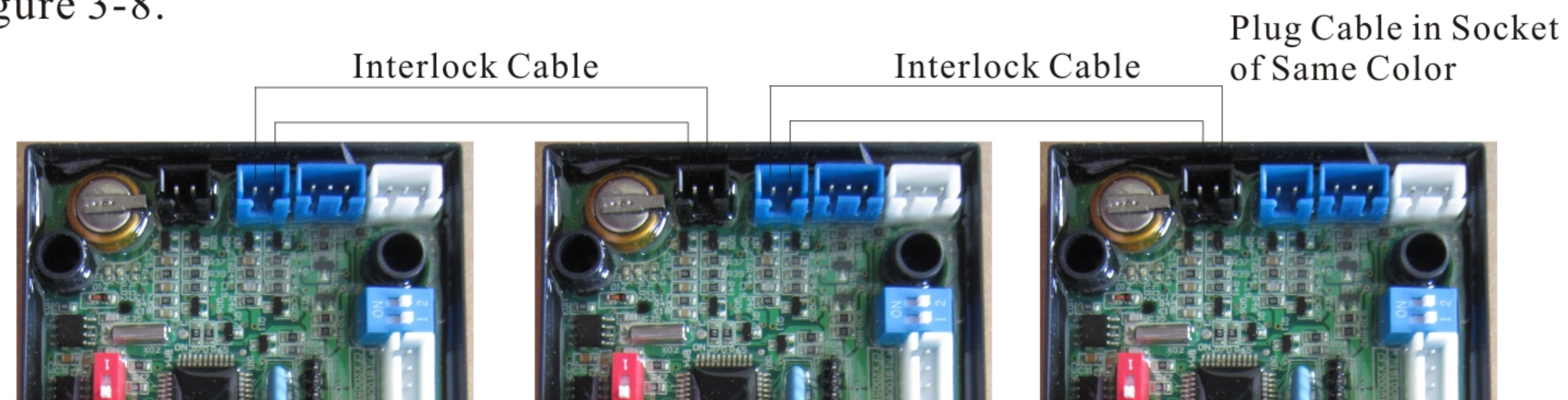
Figure 3-8 Network System Wiring with Interlock Cable
