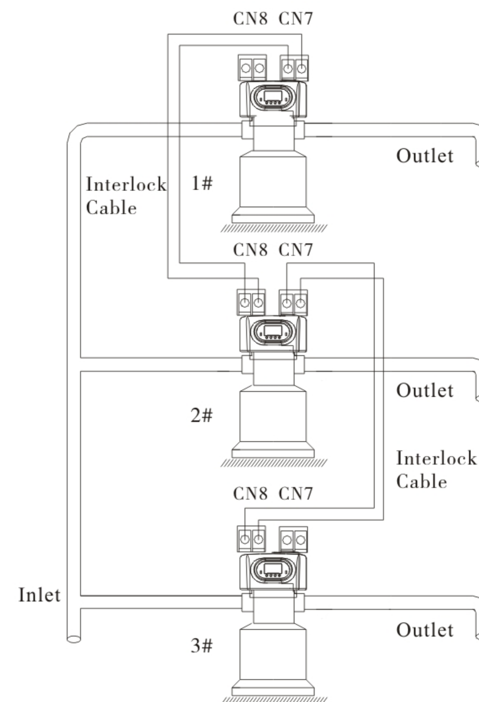
Figure3-10 Interlock system
