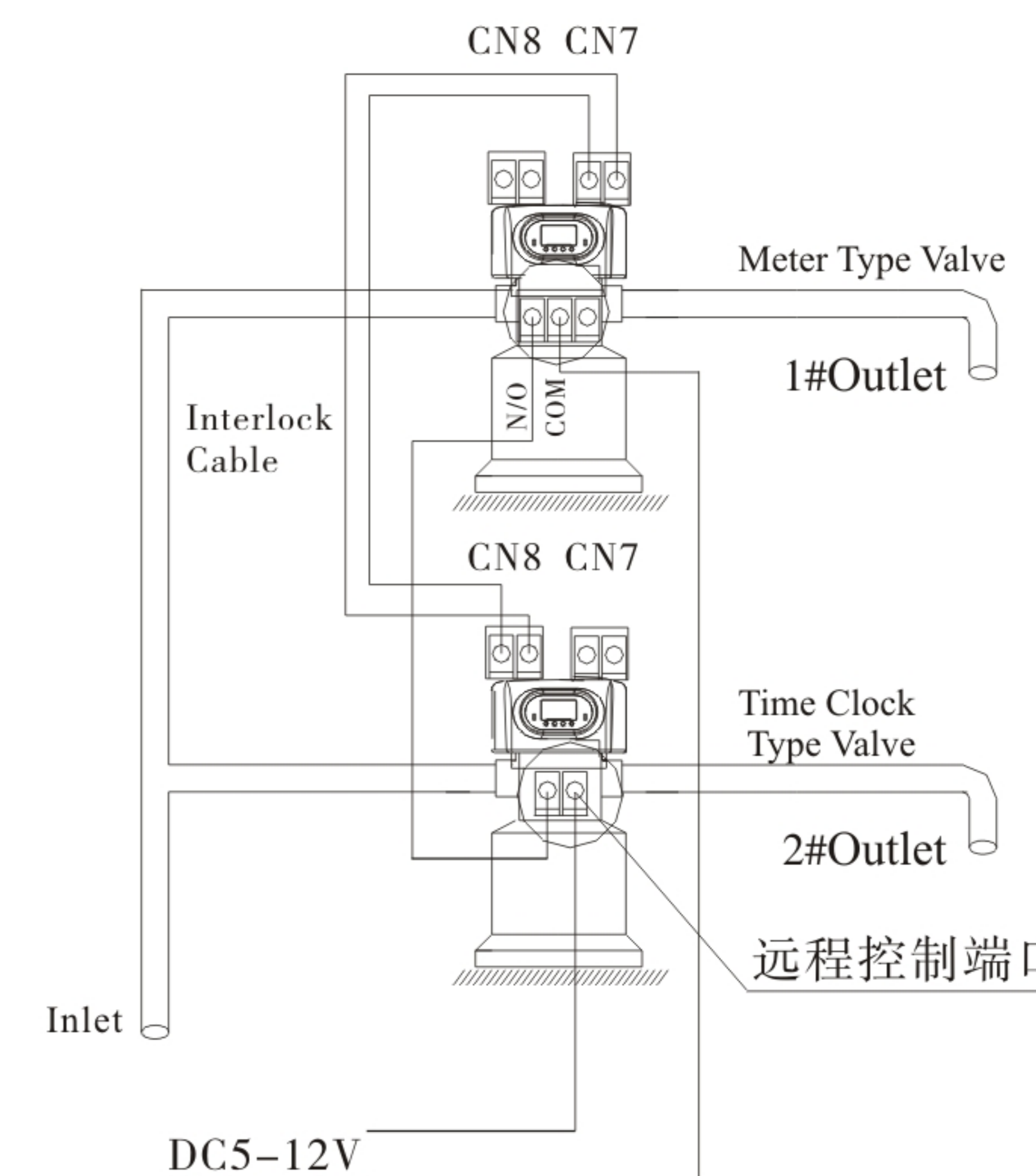
Figure3-11 Series system
