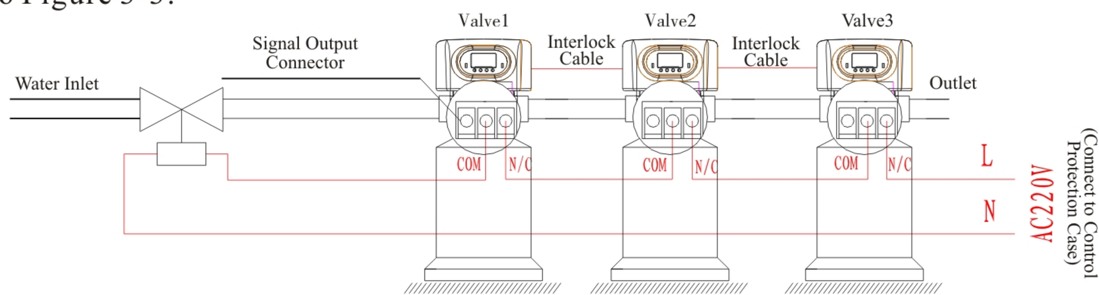
Figure 3-3 Wiring of Solenoid Valve in Inlet
