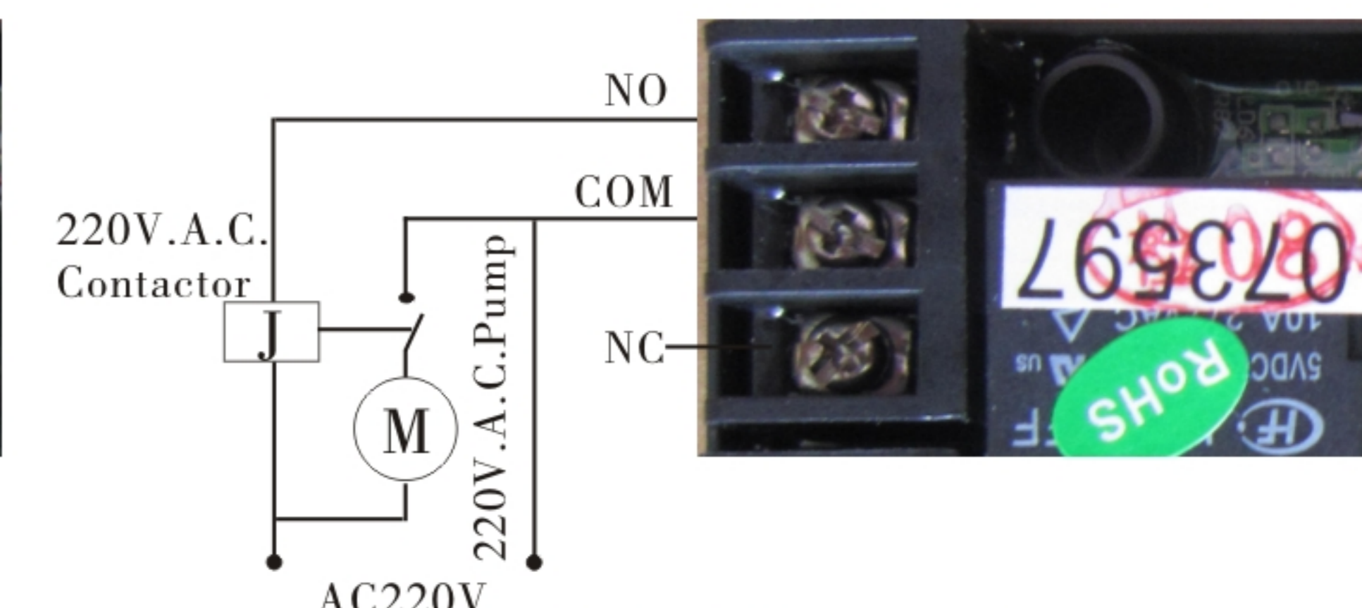
Figure 3-7Wiring of Booster pump on Inlet
