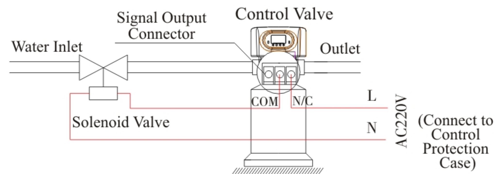
Figure 3-2 Wiring of Solenoid Valve on Inlet
