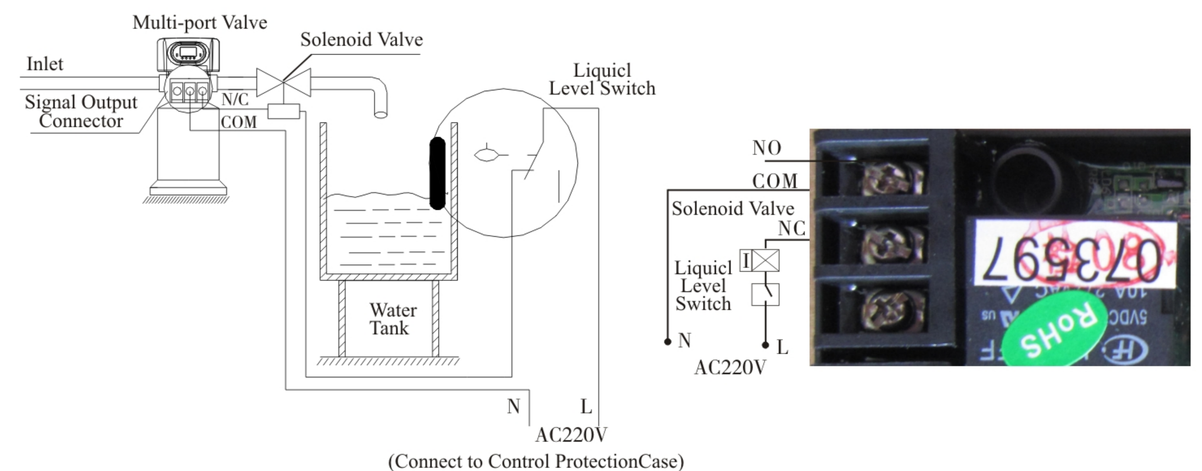
Figure 3-1 Wiring of Solenoid Valve on Outlet
