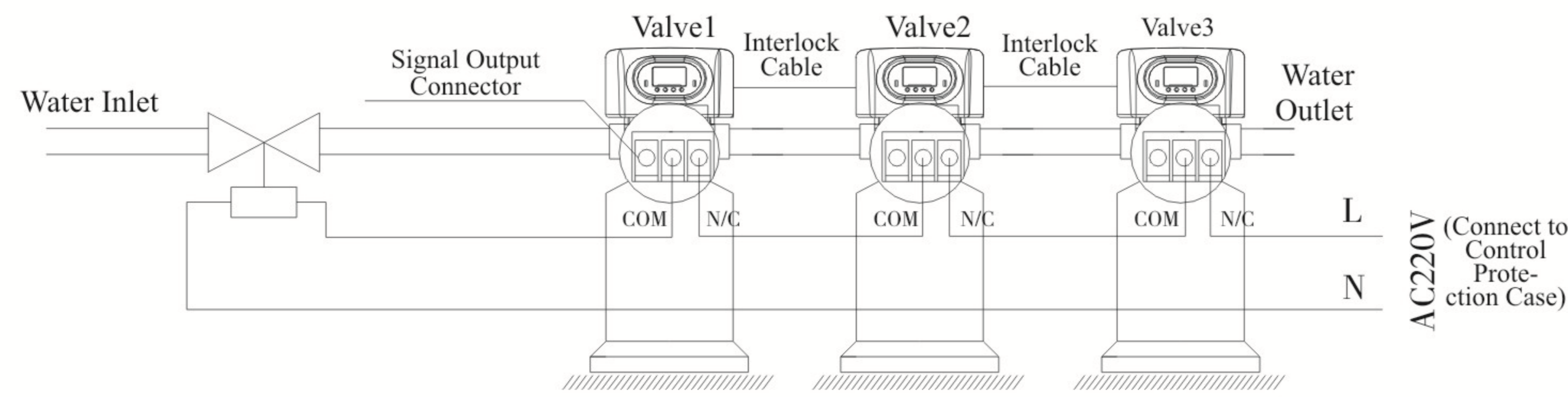
Figure 3-4 Wiring of Solenoid Valve in Inlet
