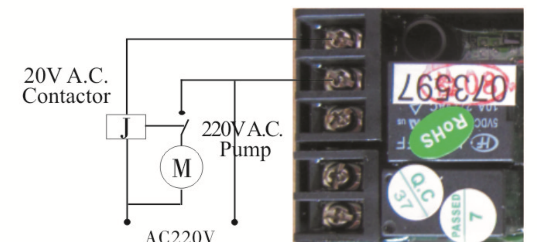
Figure 3-8 Wiring of Booster Pump on Inlet
