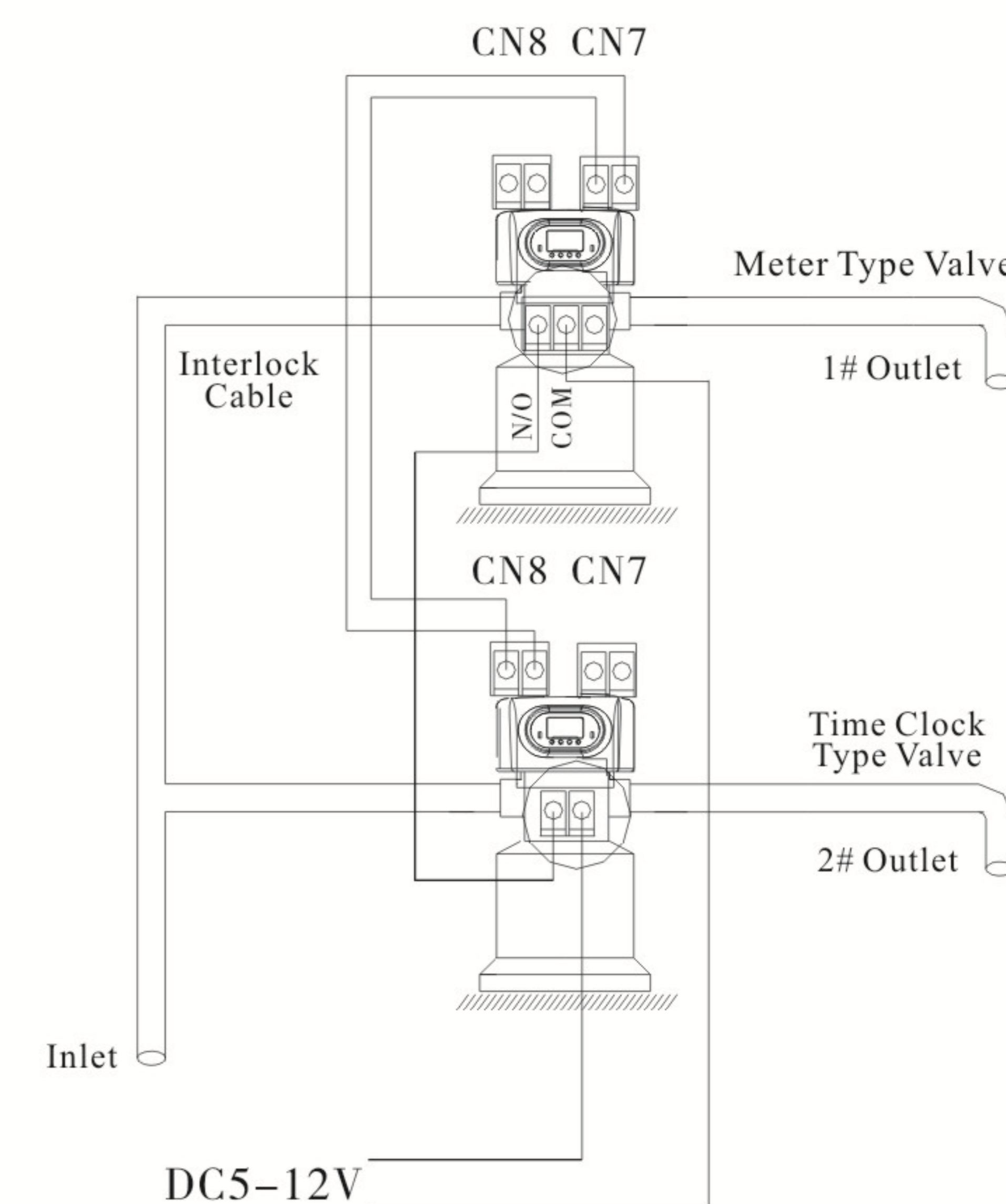
Figure 3-13 Series system
