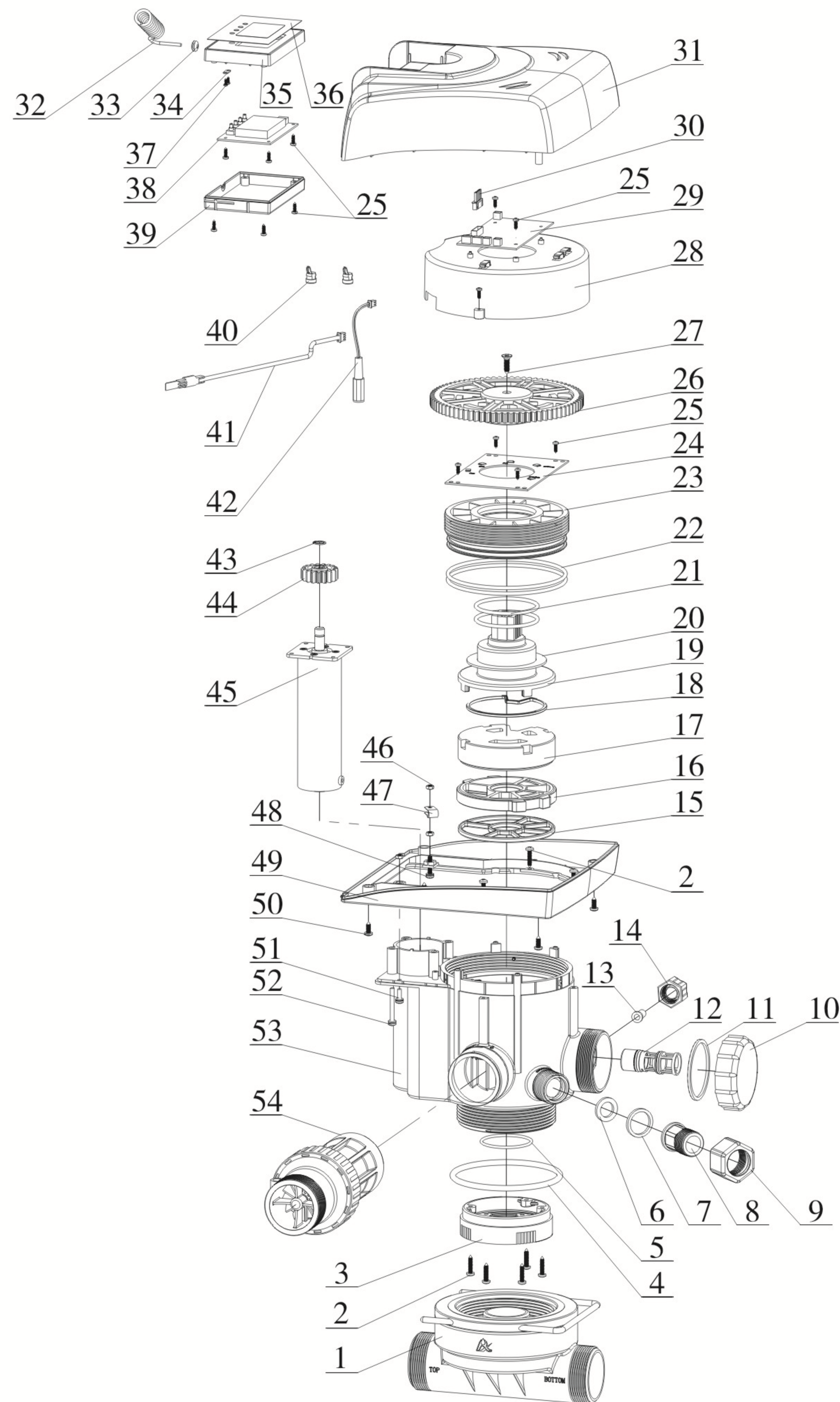
N74B3 (63510B) Structure Chart:
