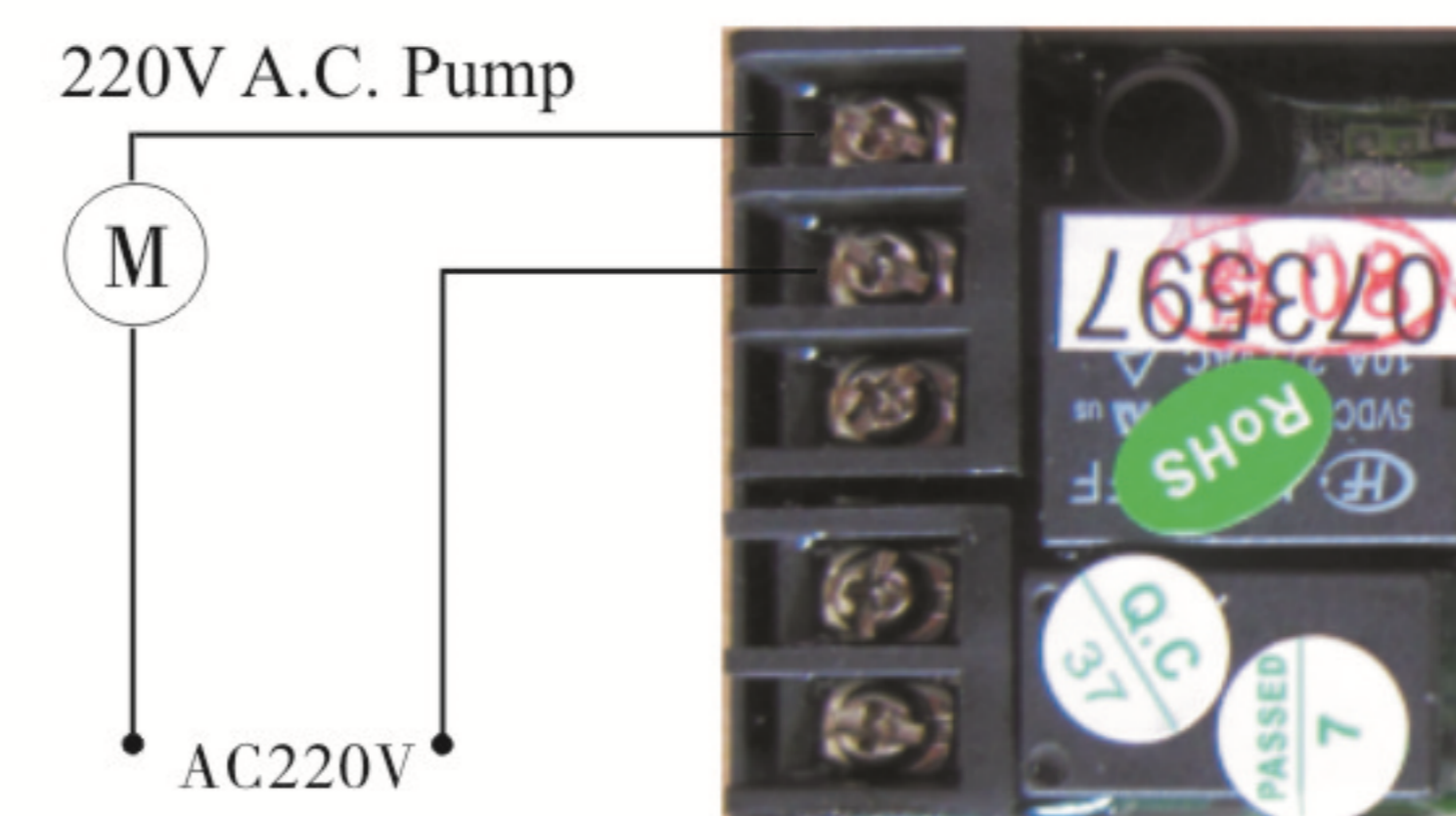
Figure 3-7Wiring of Booster Pump on Inlet
