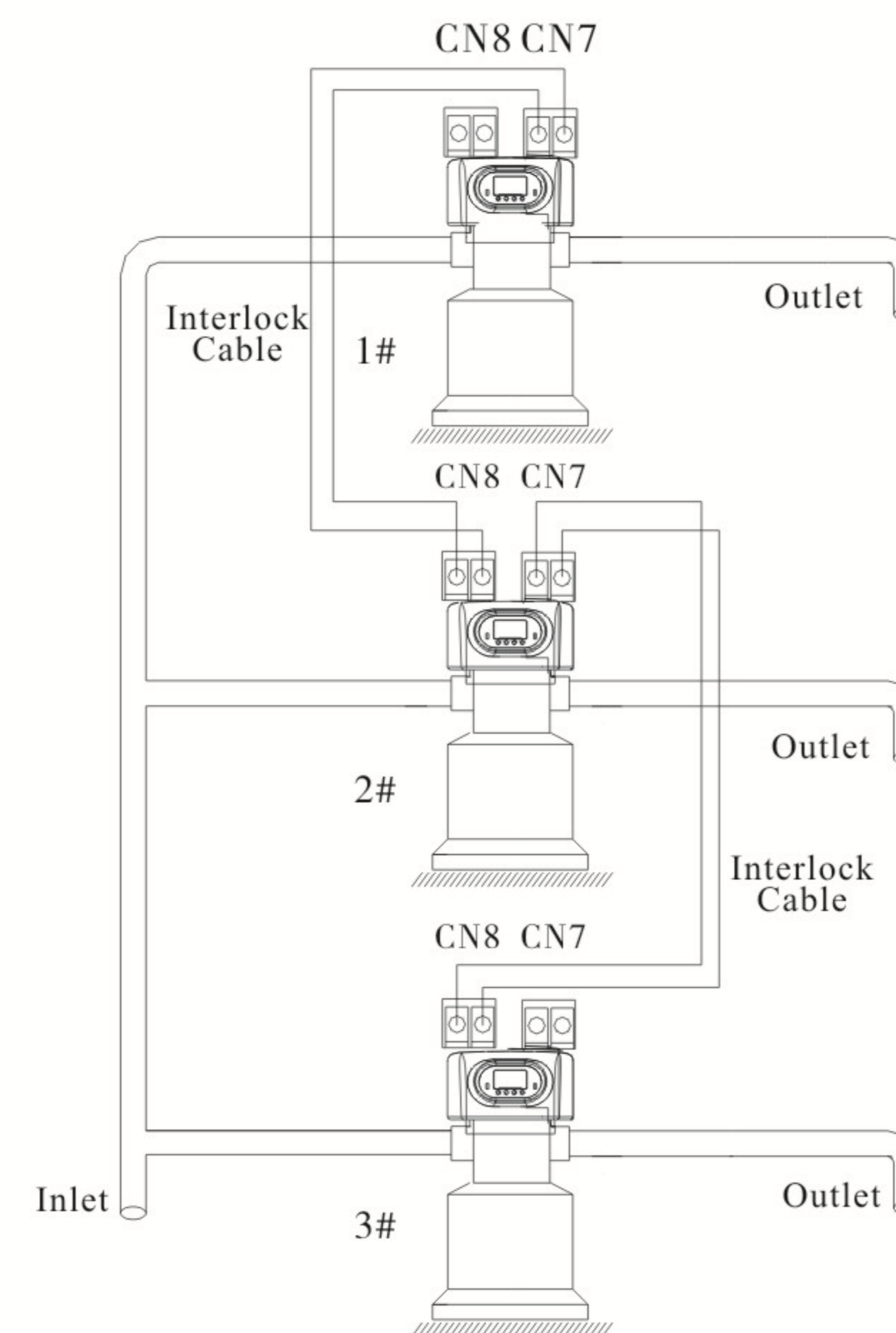
Figure 3-12 Interlock system
