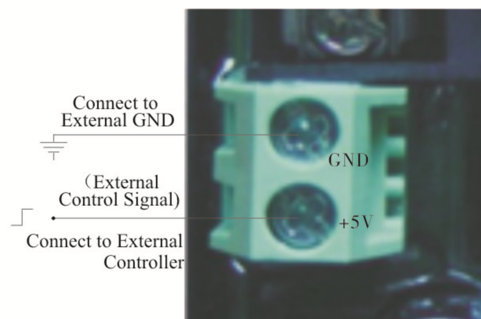
Figure 3-11 Wiring of Remote Input
