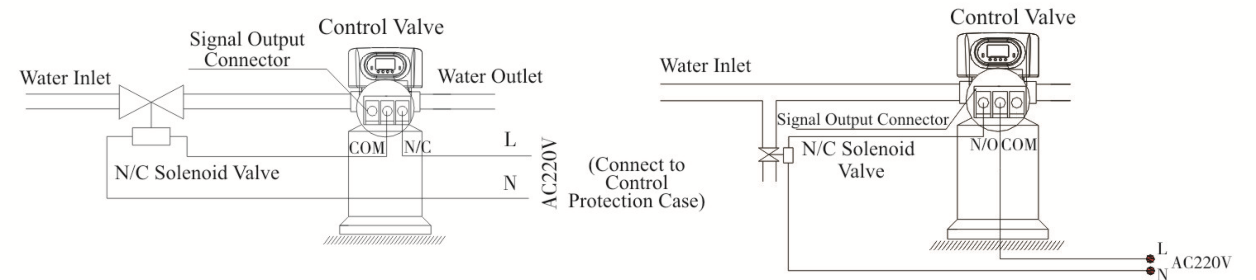
Figure 3-2 Wiring of Solenoid Valve on Inlet
