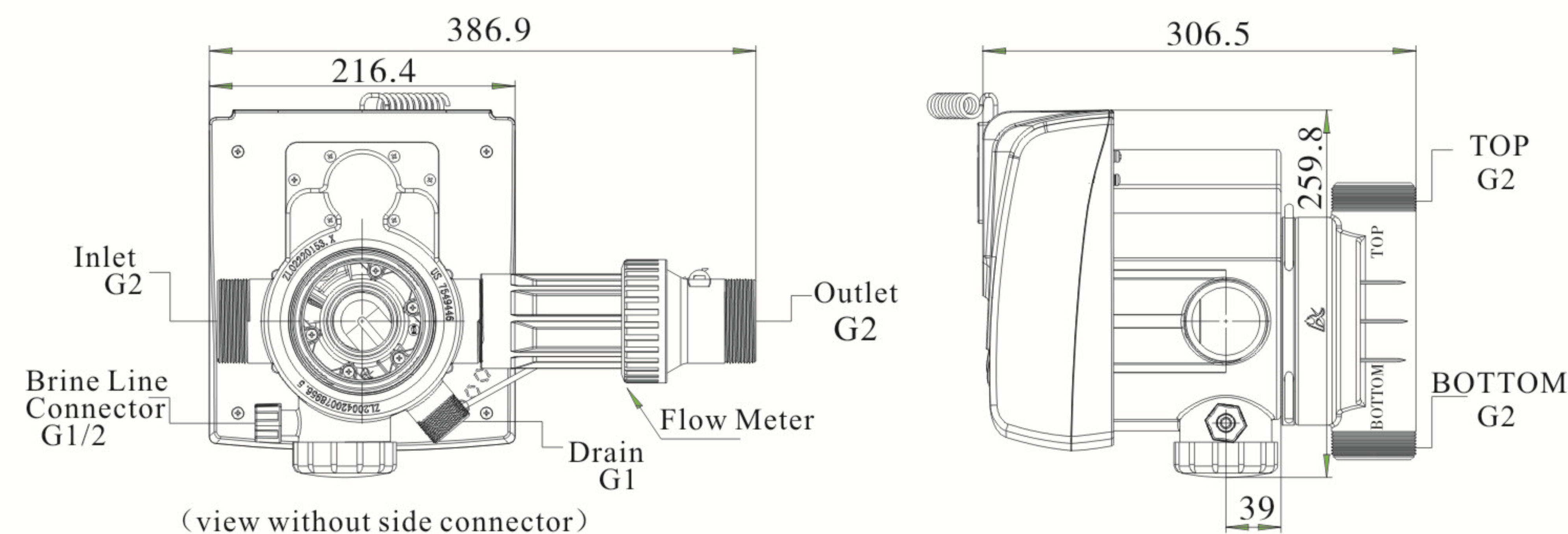
Structure Chart of N74A3 ( 63610 )
