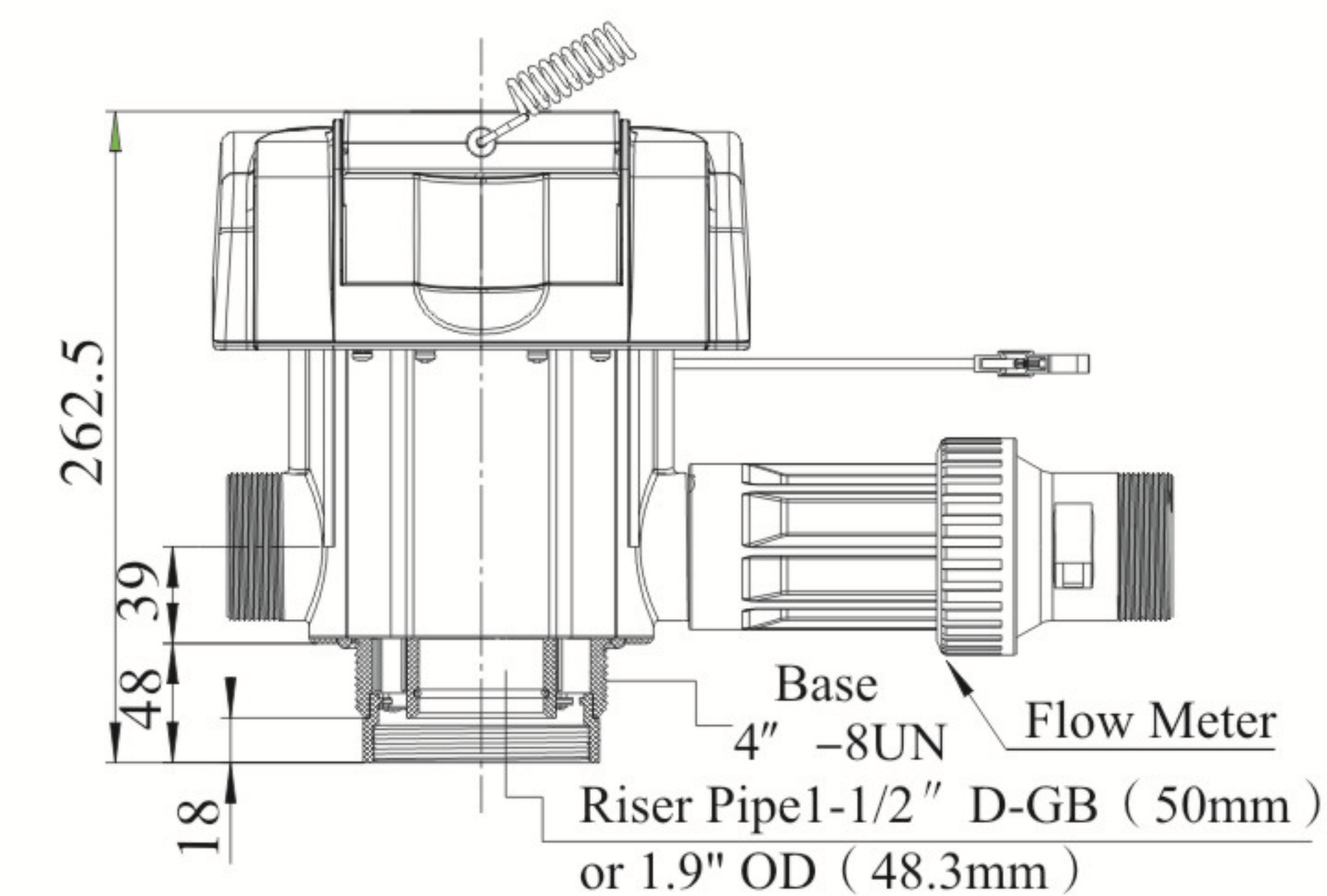
Structure Chart of N74B3 ( 63610B )
