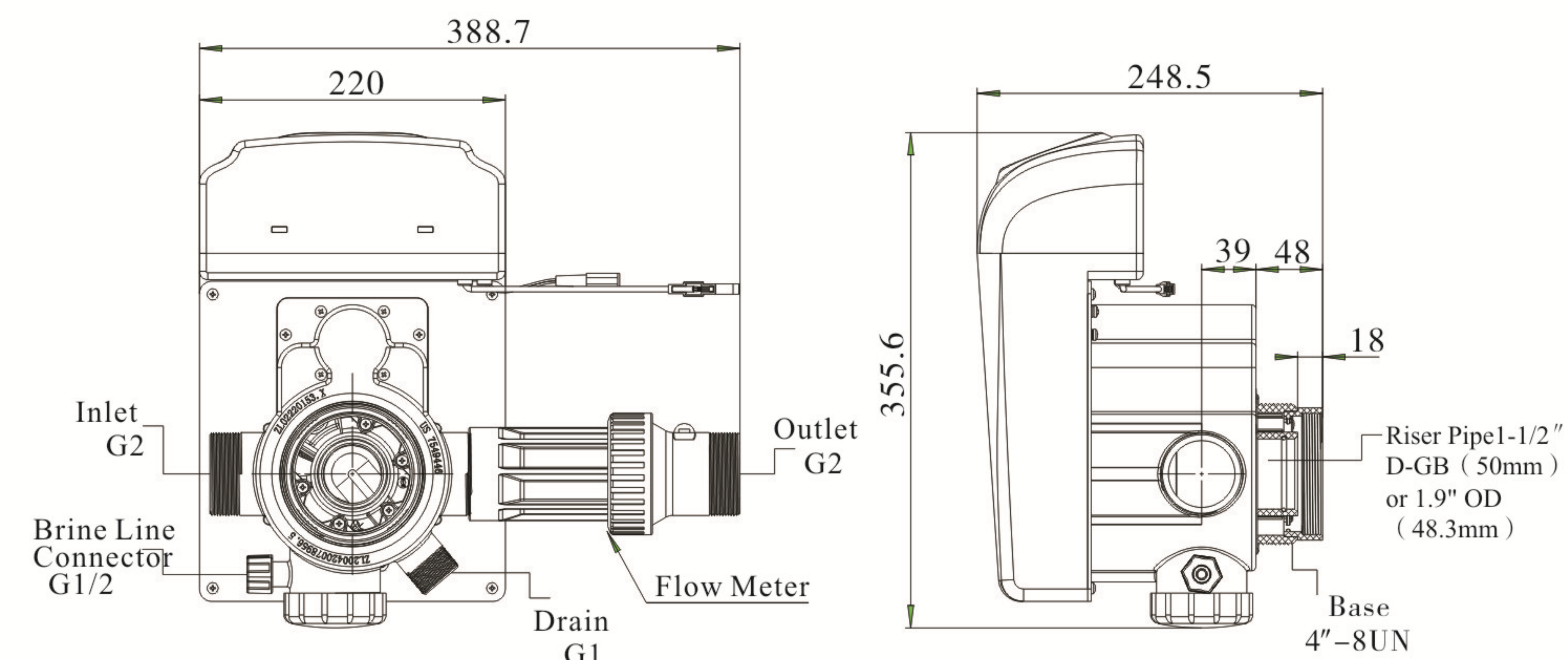
Structure Chart of N74A3 ( 63610 )
