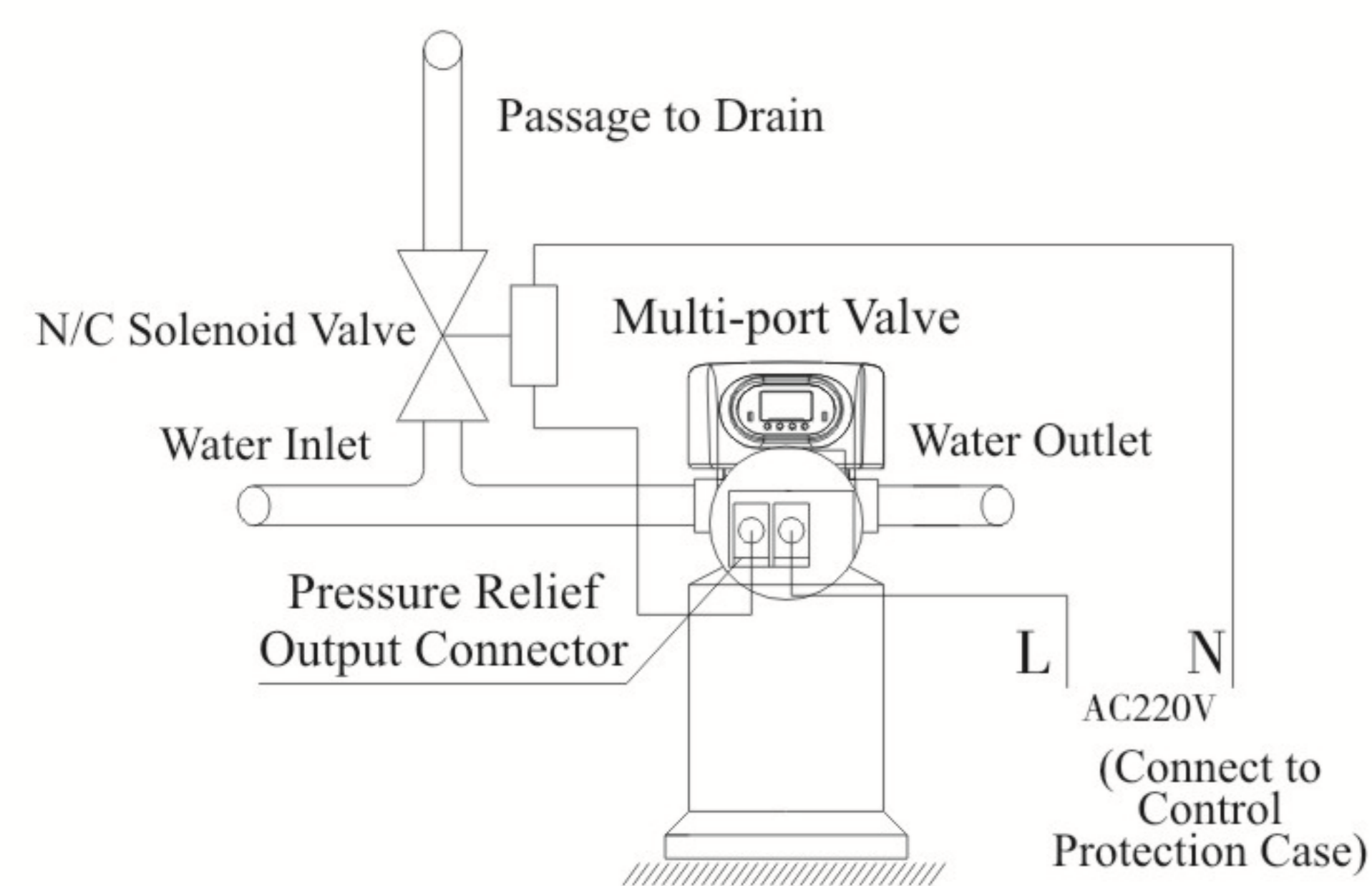
Figure 3-10 Wiring of Pressure Relief Output
