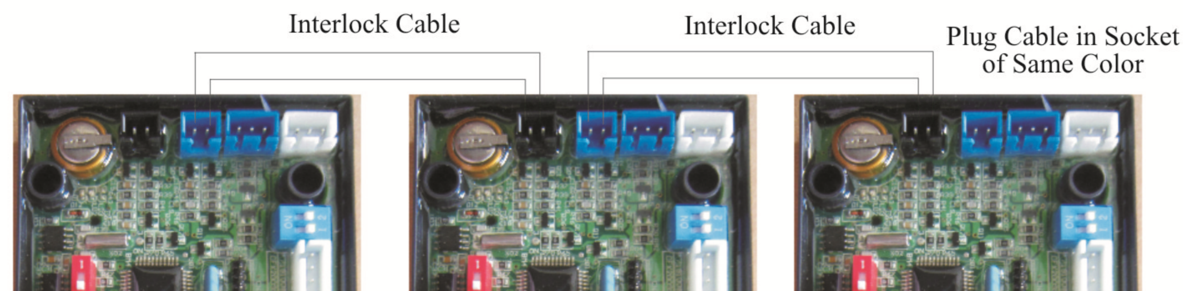
Figure 3-9 Network System Wiring with Interlock Cable
