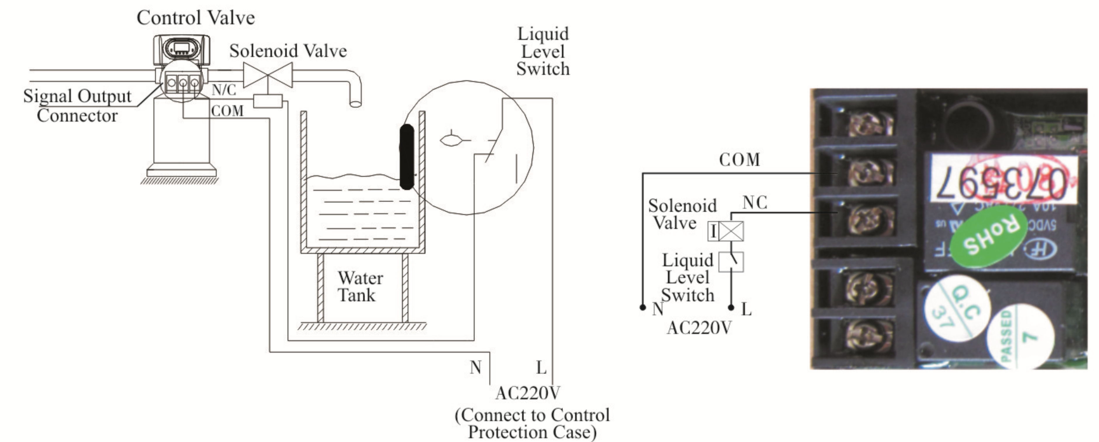
Figure3-1 Wiring of Solenoid Valve on Outlet
