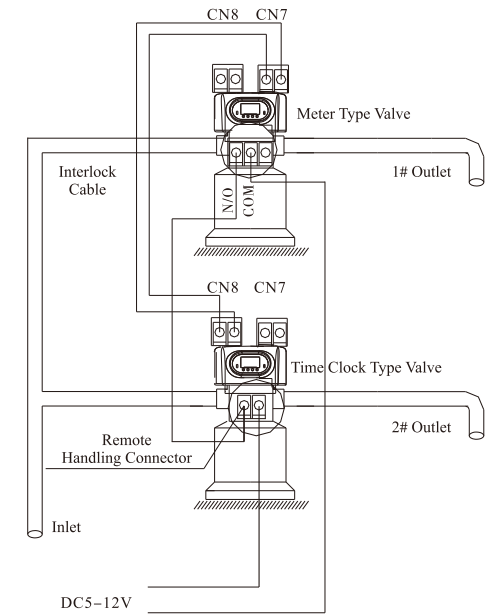
Figure 3-13 Series System
