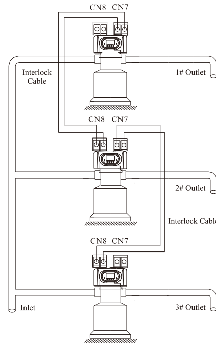
Figure 3-12 Interlock System
