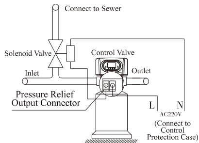
Figure 3-10 Wiring of Pressure Relief Connector
