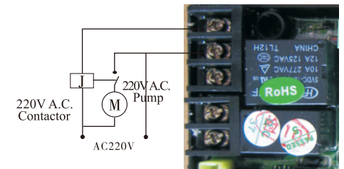
Figure 3-8 Wiring of Booster Pump on Inlet
