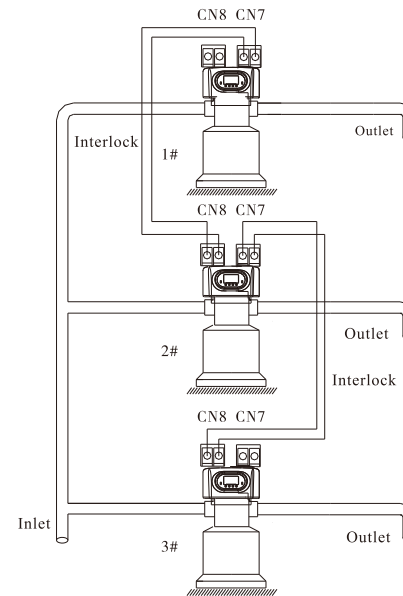
Figure 3-12 Interlock system
