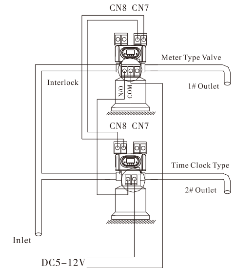
Figure 3-13 Series system
