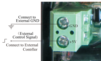
Figure 3-10 Wiring of Remote Handling Connector
