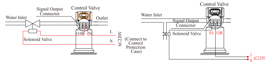
Figure 3-2 Wiring of Solenoid Valve on Inlet
