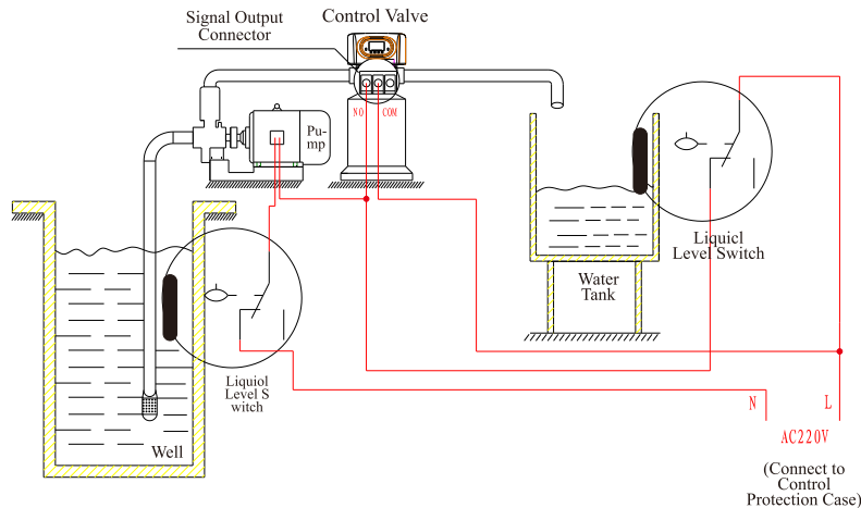
Figure 3-5 Wiring of Liquid Level Controller Controls Inlet Pump
