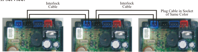
Figure 3-9 Network System Wiring with Interlock Cable
