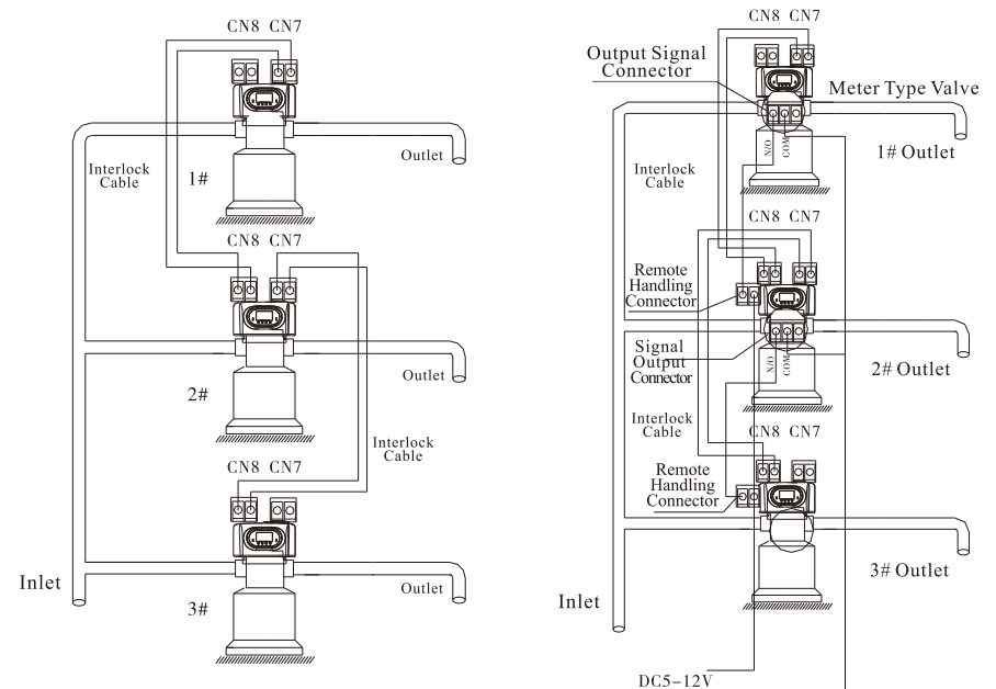
Figure 3-12 Interlock system
