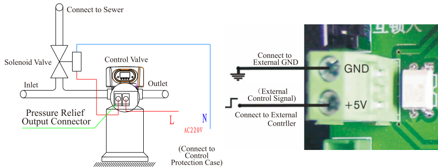
Figure 3-10 Wiring of Pressure Relief Output Figure 3-11 Wiring of Remote Input
